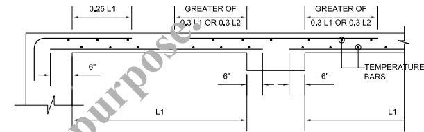
TYPICAL SLAB DETAIL
